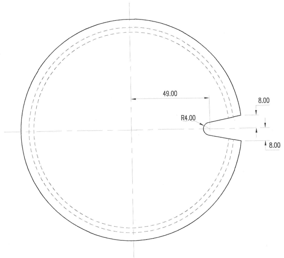
DETAIL FOR SPOON CUT OUT
