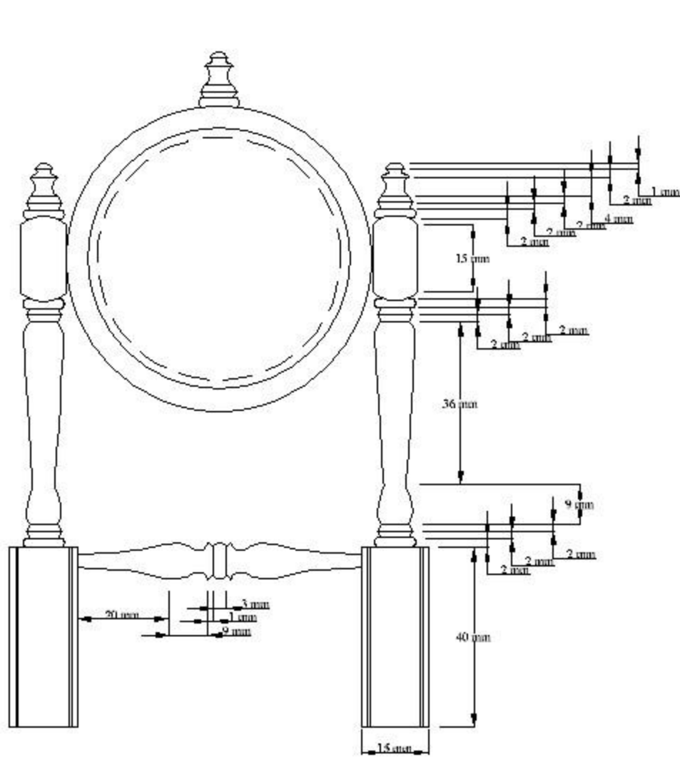
Val's Clock 58mm Clock Fitment
